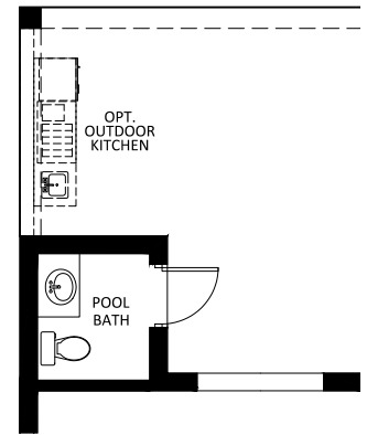
OPT. POOL BATH ADDS 46 SQ. FT. LIVING A/C I.L.O. OUTDOOR LIVING
